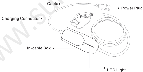
Fig. 1 Appearance details
